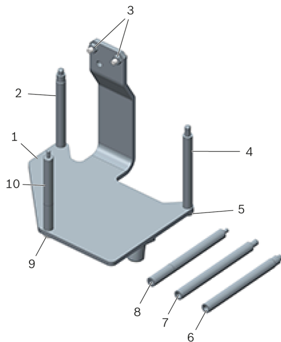
Figure 1: Engine support T40075A
