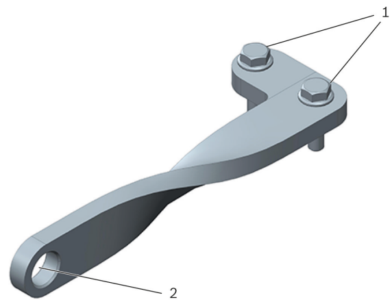
Figure 1: Holder T10339
