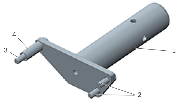
Figure 1: Gearbox support T10316
