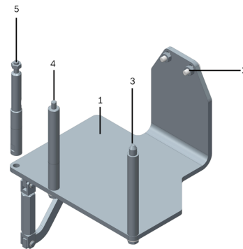
Figure 1: Engine support T10229A
