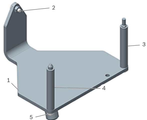
Figure 1: Engine support T10012
